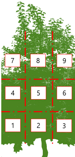
Fig. 1. Placement of water-sensitive papers in different canopy sections for spray coverage analysis. Water-sensitive papers were attached to different canopy sections of the tree to assess spray coverage. The canopy was divided into nine distinct zones: lower (0.0-1.5 m), middle (1.6-3.0 m), and upper (3.1-4.3 m) parts of the tree.
